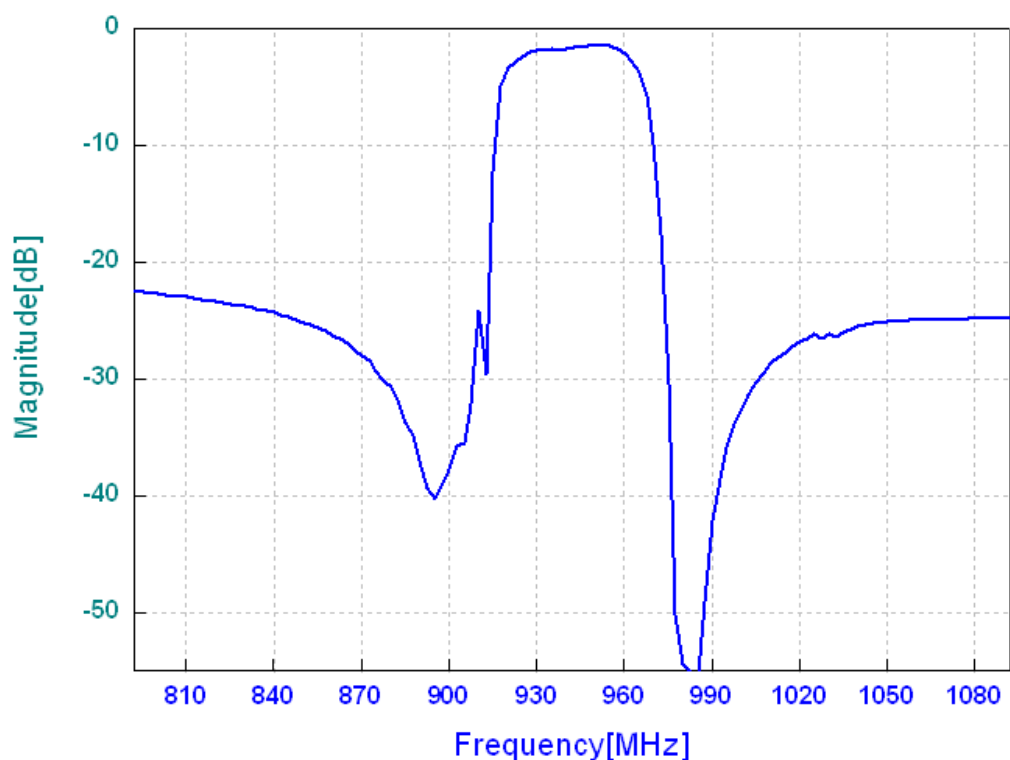
Frequency Response
